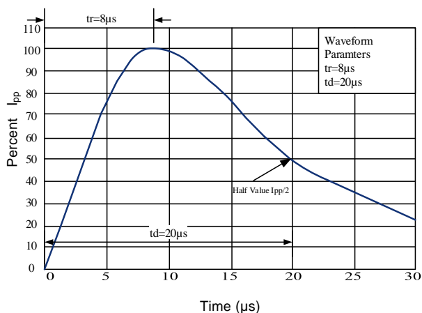
Figure 5: Pulse Waveform
